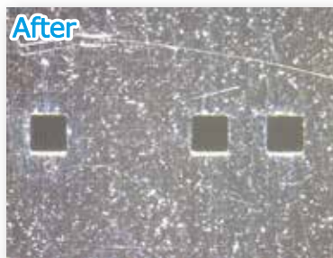
Opening : □0.18mm
